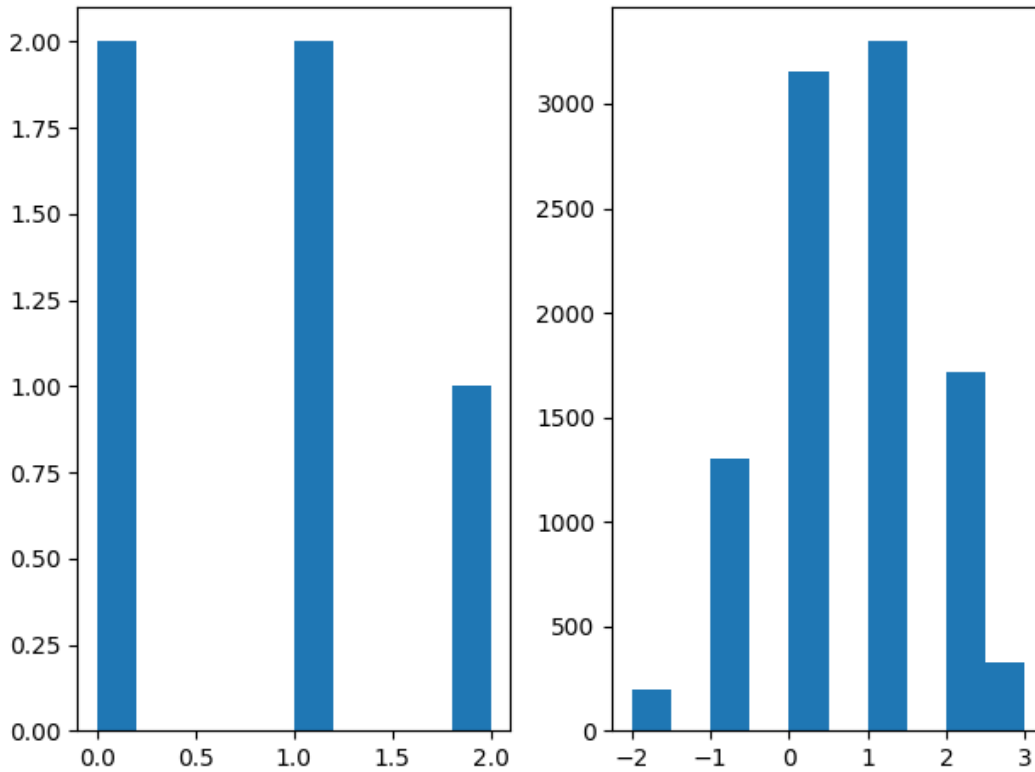
Figure 4. Distribution of reply differences (for Query #1 and #2) for the modified workflow over 5 trials (left) and over 10,000 trials (right).
