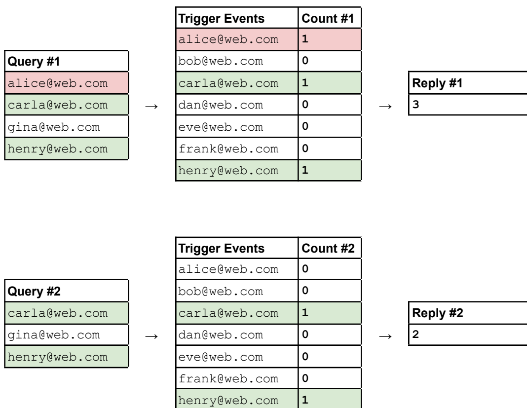
Figure 1. Diagram illustrating two attribution queries and their corresponding replies.
